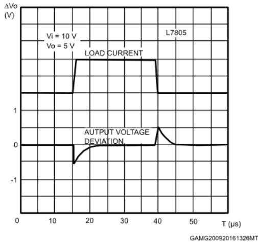
Figure 34: Load transient response
