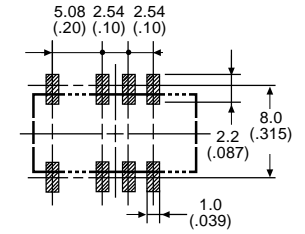
Mounting pads (Top view)
