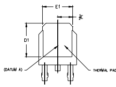
DETAIL "A" ROTATED 90°
