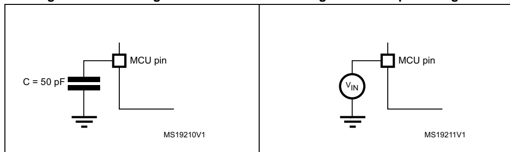
Figure 8. Pin loading conditions
