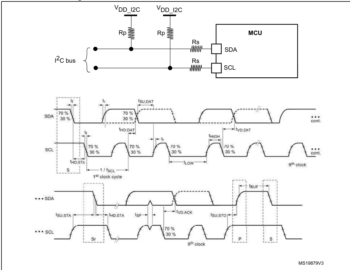
Figure 22. I2C bus AC waveforms and measurement circuit
