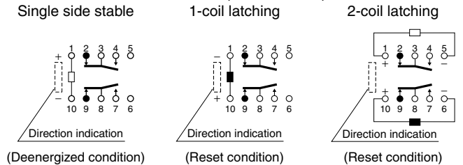
Schematic (Bottom view)
