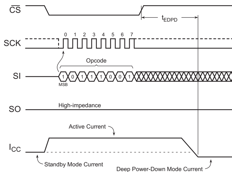
Figure 9-1. Deep Power-Down
