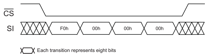
Figure 12-1. Software Reset
