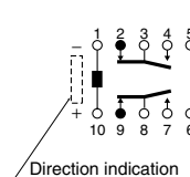
1-coil latching
