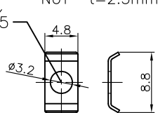
SMALL WASHER
