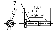
Short BOLT
