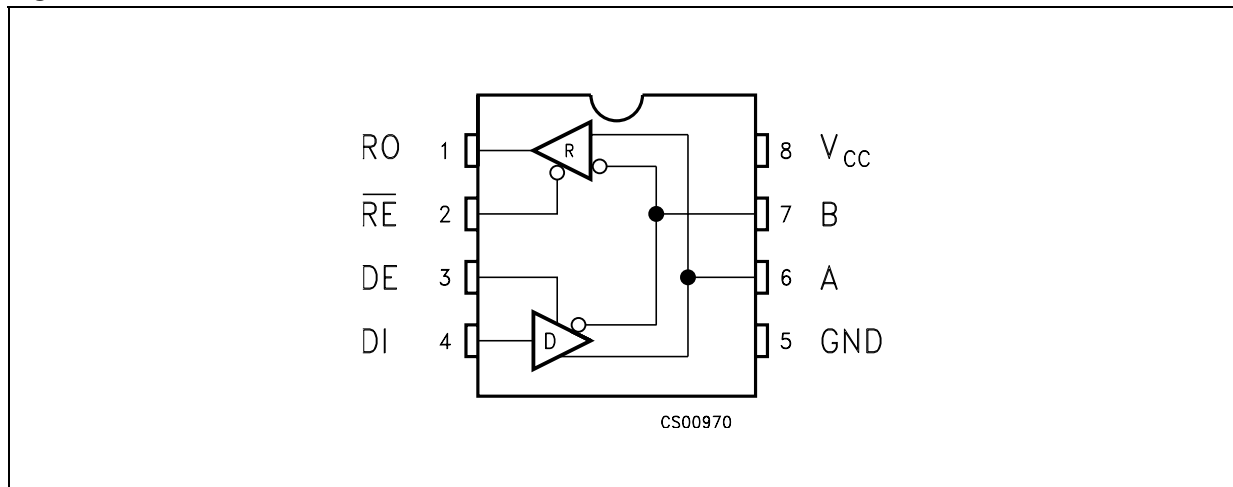
Figure 2. Pin connections
