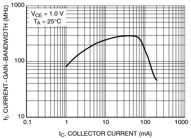
Figure 22. Current-Gain-Bandwidth Product
