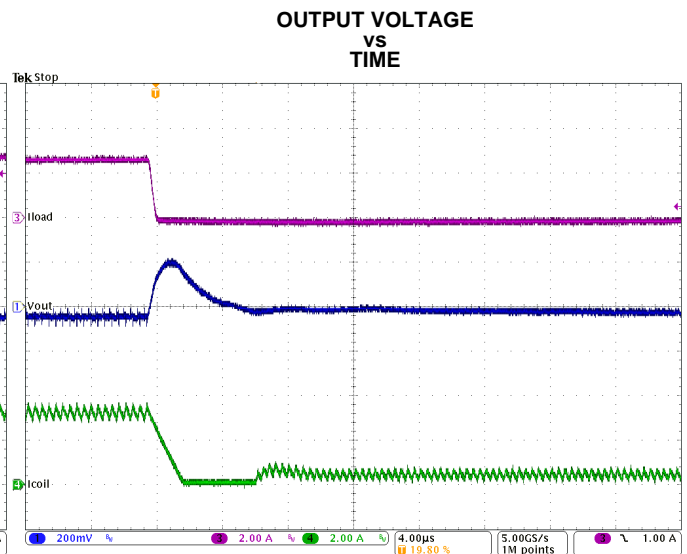
Figure 32. Load Transient Response of Figure 30, falling edge
