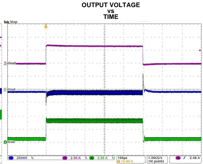
Figure 30. Load Transient Response ( I_{OUT}= 0.5 to 3 to 0.5 A, V_{IN}=12V , V_{OUT}=3.3V )
