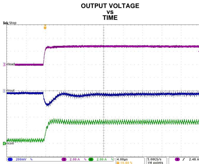
Figure 31. Load Transient Response of Figure 30, rising edge
