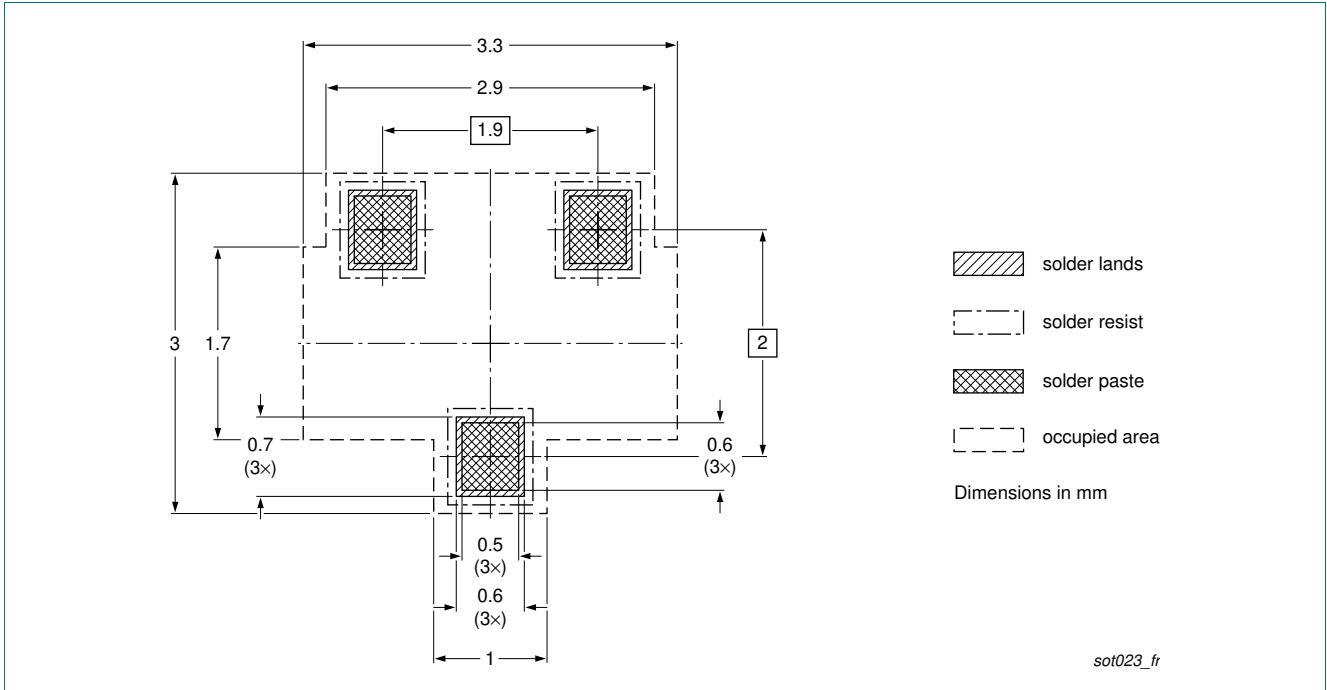
Fig 14. Reflow soldering footprint for SOT23 (TO-236AB)
