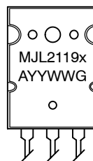
TO-3PBL (TO-264) CASE 340G
