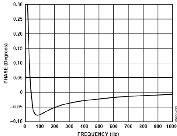
Figure 23. Phase Error Between Channels (0 Hz to 1 kHz)
