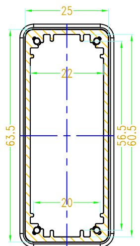
SEC B-B
