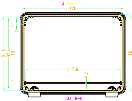
SEC B-B
