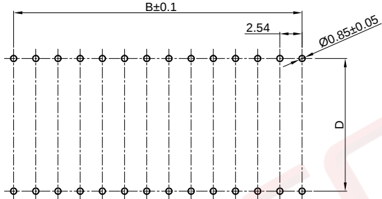
Recommended PCB layout(Tolerance:±0.05)
